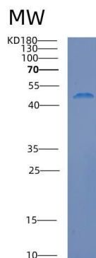
Figure 2. SDS-PAGE
