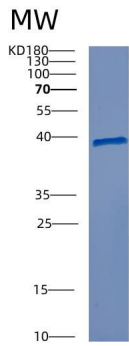
Figure . SDS-PAGE
