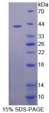
Figure 1. SDS-PAGE
