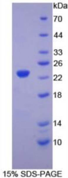
Figure 2. SDS-PAGE
