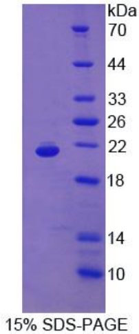
Figure 1. SDS-PAGE
