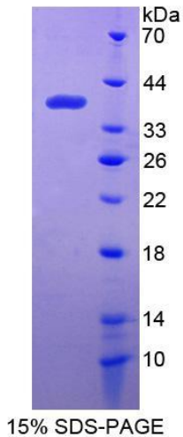
Figure 1. SDS-PAGE
