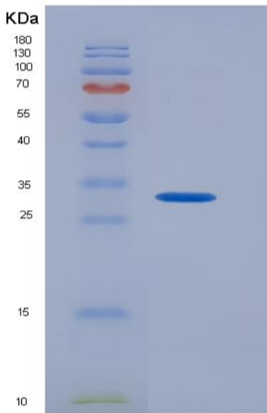
Figure 2. SDS-PAGE
