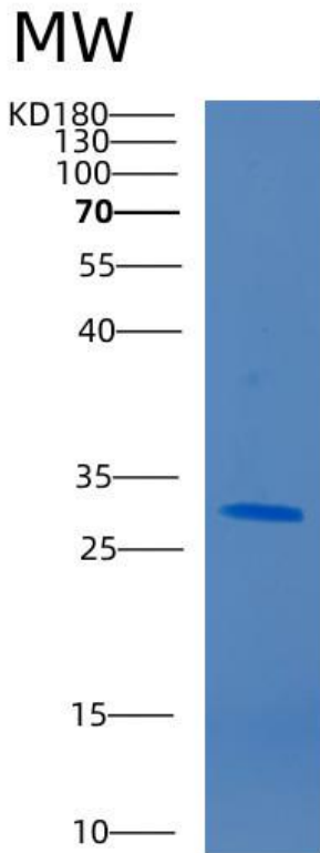
Figure 1. SDS-PAGE
