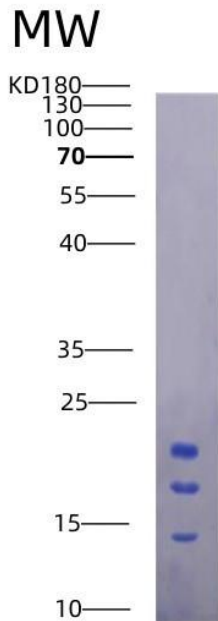
Figure 2. SDS-PAGE
