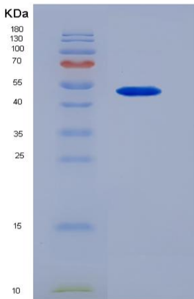
Figure 2. SDS-PAGE
