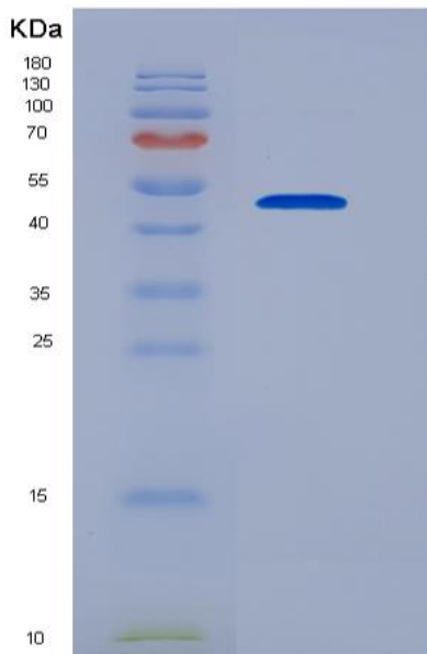
Figure 2. SDS-PAGE
