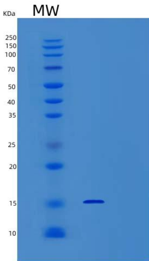
Figure 2. SDS-PAGE
