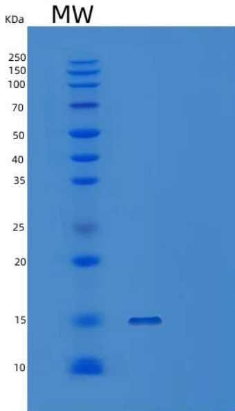
Figure 1. SDS-PAGE
