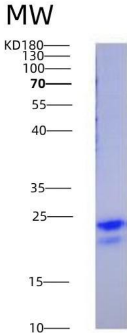
Figure 1. SDS-PAGE
