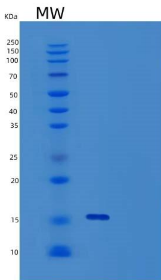
Figure 2. SDS-PAGE
