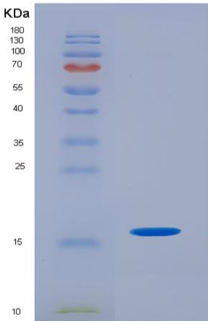
Figure 1. SDS-PAGE
