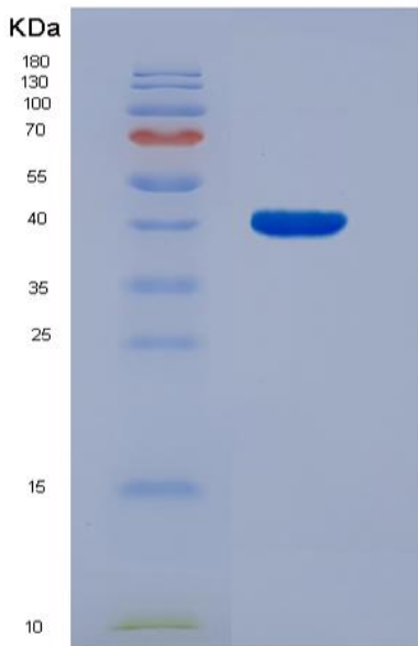
Figure 1. SDS-PAGE
