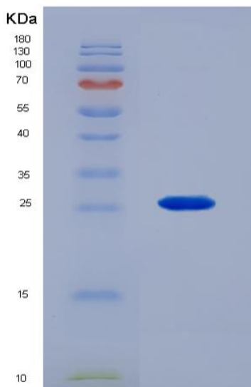
Figure 2. SDS-PAGE
