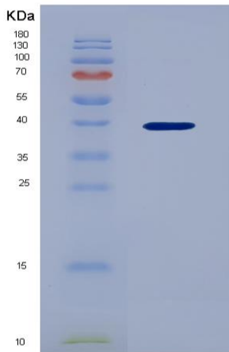
Figure 2. SDS-PAGE
