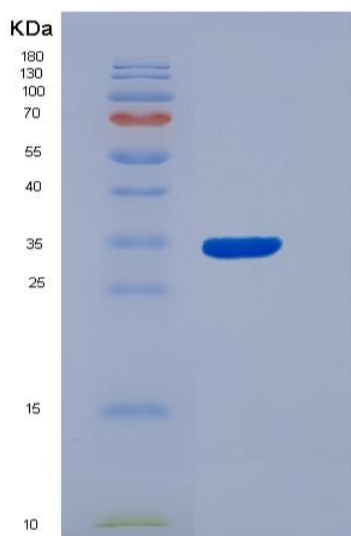
Figure . SDS-PAGE
