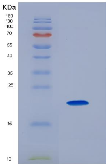
Figure 1. SDS-PAGE
