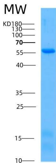
Figure . SDS-PAGE
