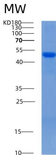
Figure 2. SDS-PAGE
