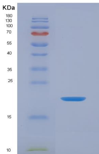
Figure 2. SDS-PAGE
