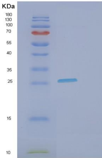
Figure . SDS-PAGE
