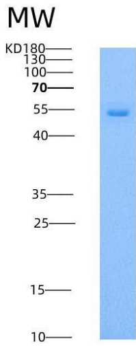
Figure 1. SDS-PAGE
