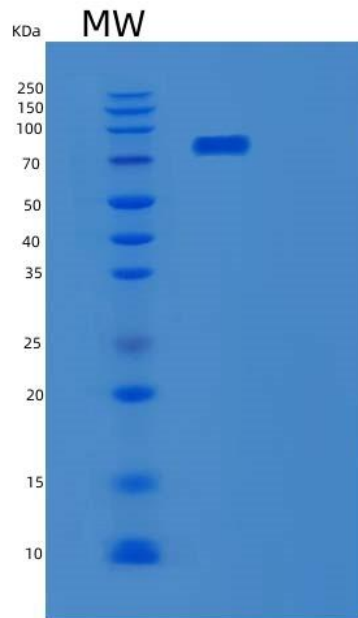
Figure . SDS-PAGE
