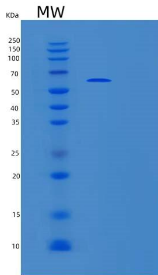
Figure . SDS-PAGE
