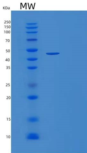
Figure . SDS-PAGE
