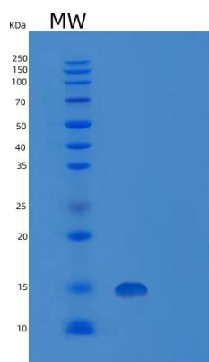
Figure . SDS-PAGE
