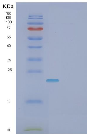
Figure . SDS-PAGE
