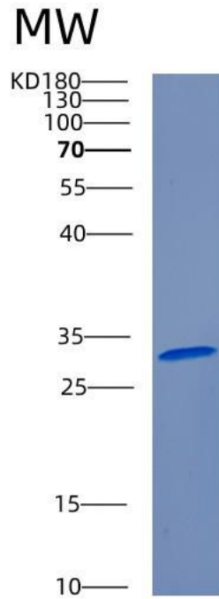
Figure . SDS-PAGE
