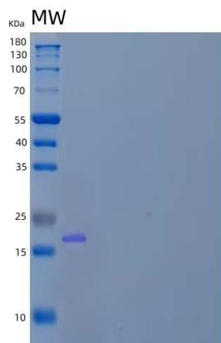
Figure . SDS-PAGE
