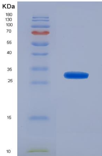
Figure 1. SDS-PAGE
