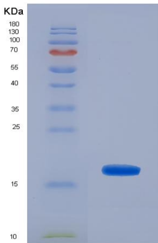
Figure 1. SDS-PAGE
