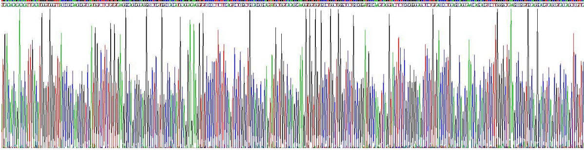
Figure1:Gene Sequencing(extract)
