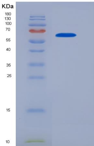
Figure 1. SDS-PAGE
