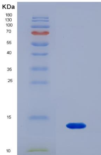
Figure 2. SDS-PAGE
