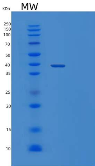
Figure 1. SDS-PAGE
