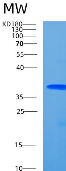
Figure 1. SDS-PAGE
