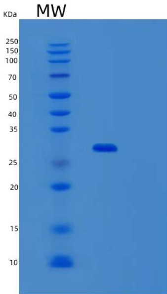
Figure 1. SDS-PAGE
