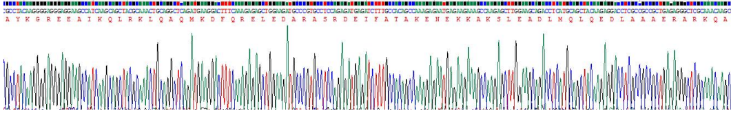
Figure 1. Gene Sequencing (Extract)
