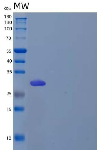
Figure . SDS-PAGE
