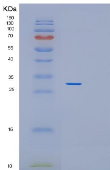
Figure 2. SDS-PAGE
