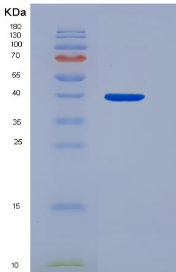
Figure 1. SDS-PAGE
