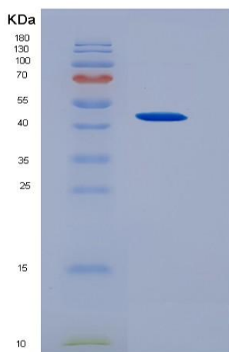
Figure . SDS-PAGE
