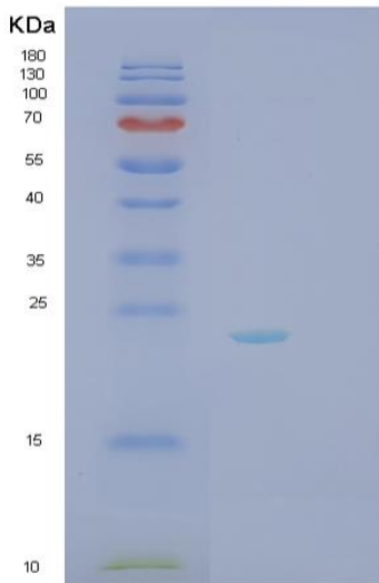
Figure 1. SDS-PAGE
