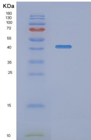
Figure . SDS-PAGE
