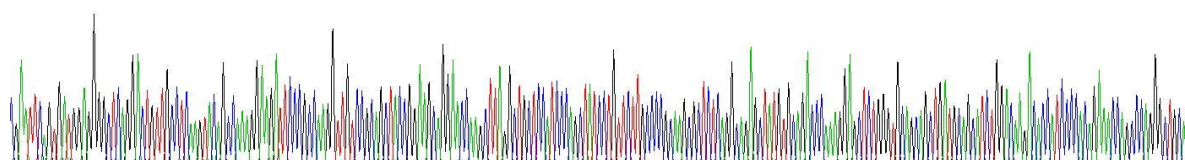
Figure 1. Gene Sequencing (Extract)
