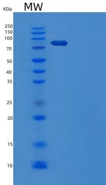
Figure . SDS-PAGE
